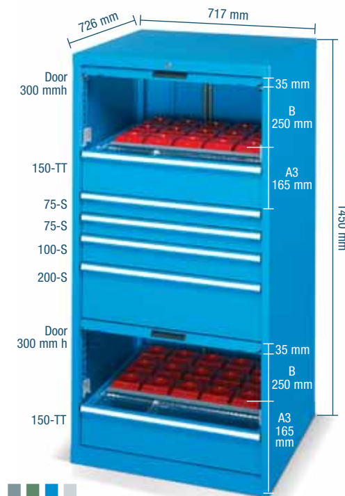
■ The door can be closed by the edge of the lower drawer handle (ref. Y)
