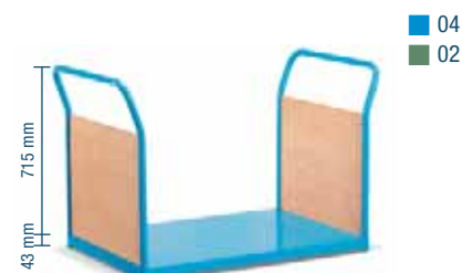
Steel base
