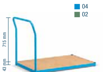
Wooden base
