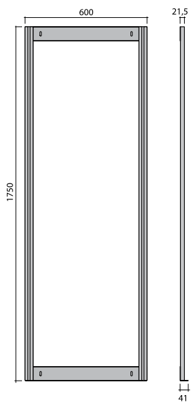
Ord. no. F PG 0550 00 01 measurements in mm
