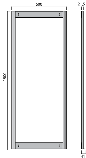
Ord. no. F PG 0540 00 01 measurements in mm
