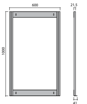
Ord. no. F PG 0530 00 01 measurements in mm
