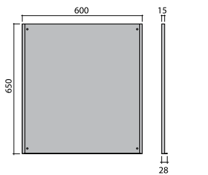
Ord. no. F PG 0430 00 01 measurements in mm
