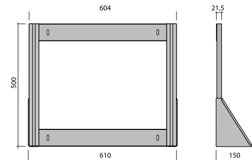
ORD. NO. F PG 0320 00 01 - measurements in mm
