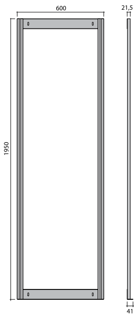
Ord. no. F PG 0560 00 01 measurements in mm
